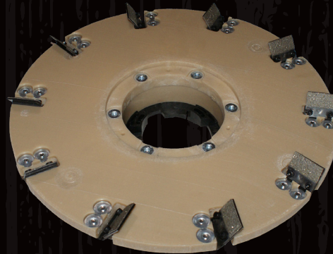
Mastic Removal Tool 56383926 use with Epoch HD, RS-16DC, Sander 1600, Phoenix
