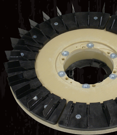
Concrete Prep Tool 56383930 use with Epoch HD, RS-16DC, Sander 1600, Phoenix
