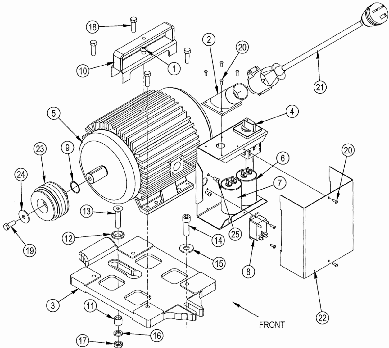
MOTOR ASSY [MODEL 07120A]
