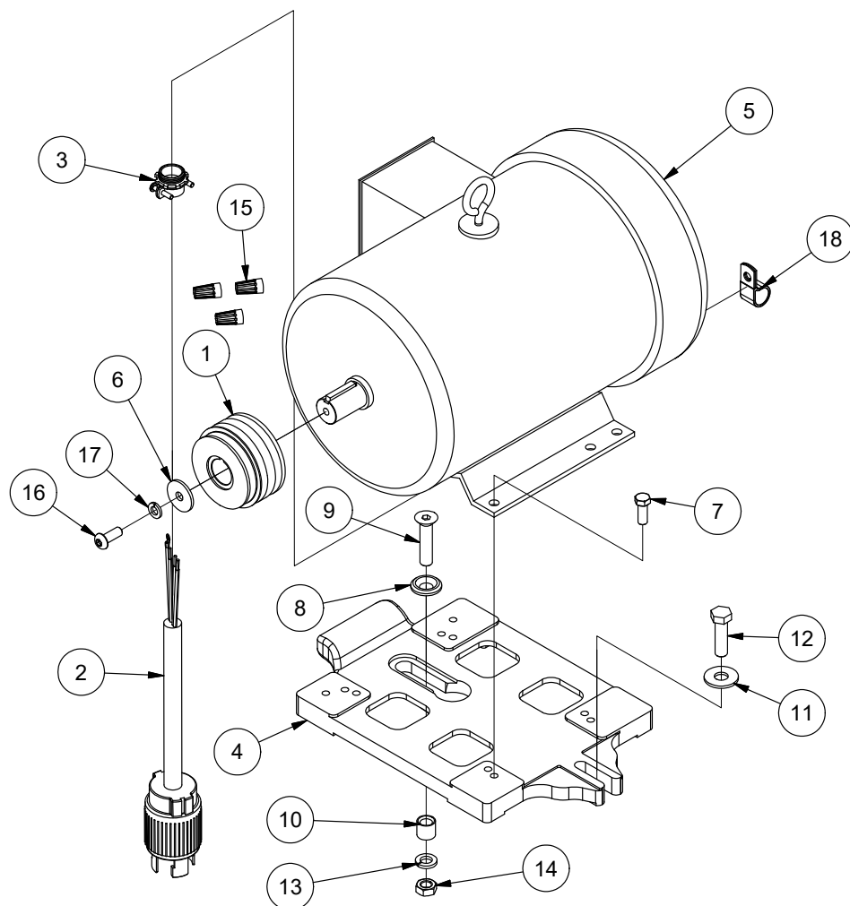
MOTOR ASSY [MODEL 07108B]
